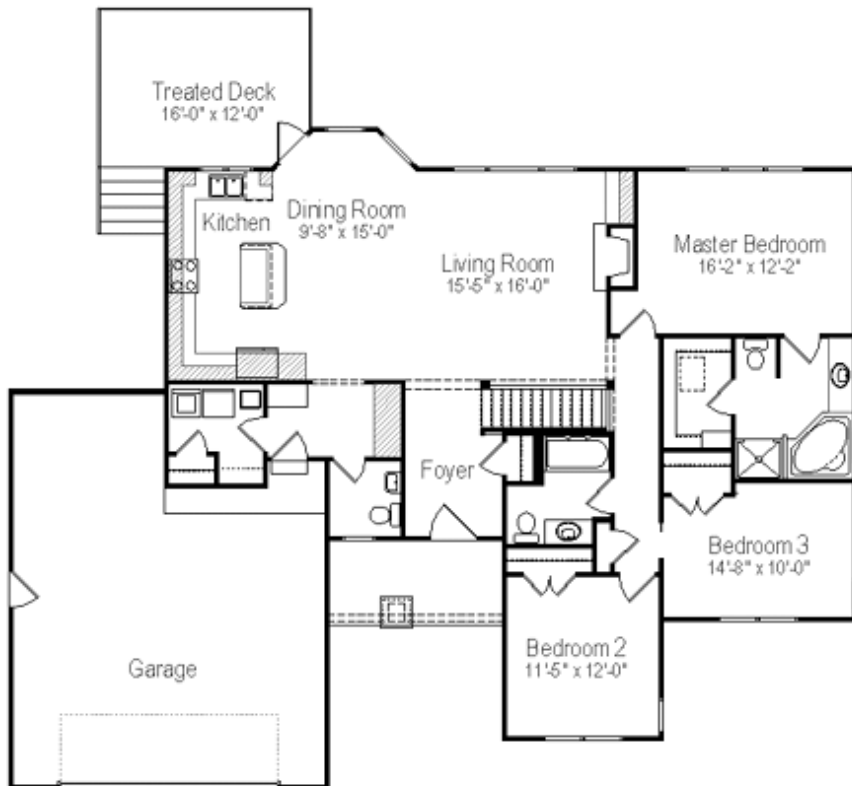
Main Floor 1,686 sq. ft.
