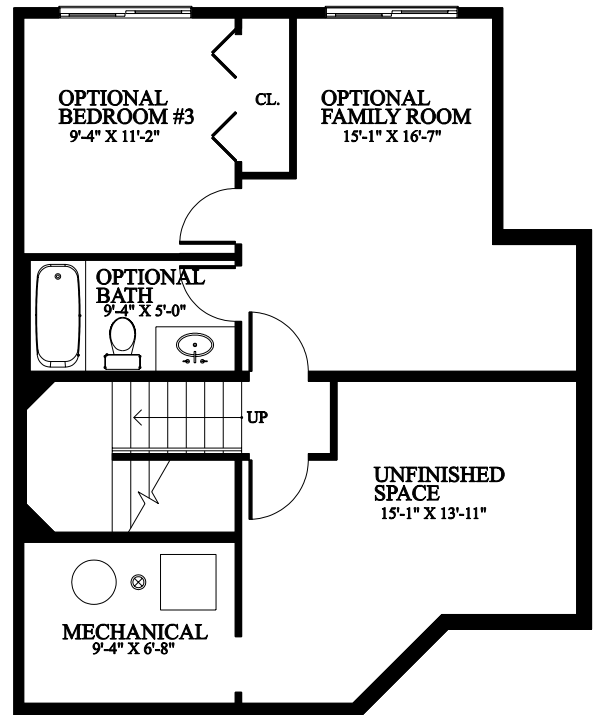
LOWER LEVEL FLOOR PLAN (WITH OPTIONAL FINISHES SHOWN) 689 SQ. FT. - FUTURE EXPANSION
